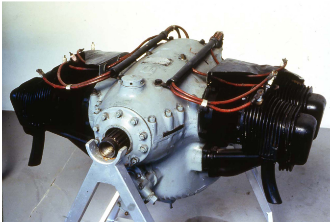
1940 CNA D light aircraft engine
