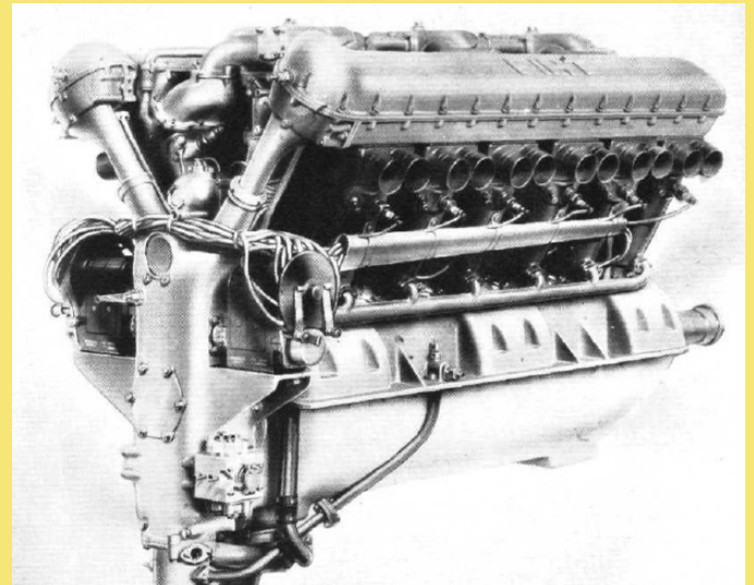
1926 Fiat AS.2, 31L V-12 - From Wikipedia
