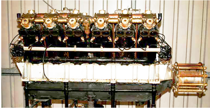
1917 Fiat A.14, 57L V-12 - from Wikipedia
